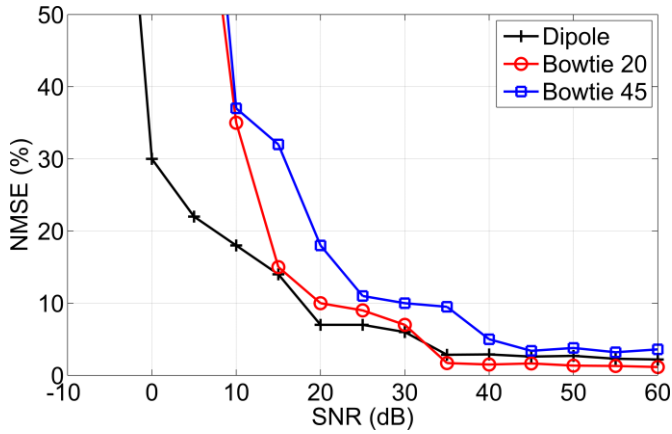
a. Matrix Pencil method
