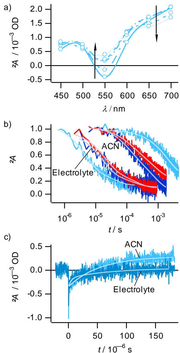
Figure 6. Temporal evolution of the transient absorption spectrum of a PAB-1 sensitized \text{TiO}_2 film in acetonitrile (ACN), showing the decay of the radical cation signature at 650 nm and the formation of the dication signal at 550 nm (bold line 10 \mu\text{s} and dotted line 180 \mu\text{s} after excitation). b) Normalized transient absorption decay at 650 nm of the radical cation of PAB-1 (light blue), PAB-2 (blue), or PAB-3 (red) in ACN and in the presence of an iodide/tri-iodide redox electrolyte. Continuous lines drawn on top of experimental data are single exponential fits with the following time constants: In ACN: \tau = 2.3 ms ( PAB-1 ), \tau = 256 \mu\text{s} ( PAB-2 ), \tau = 494 \mu\text{s} ( PAB-3 ). In electrolyte: \tau = 7 \mu\text{s} ( PAB-1 ), \tau = 18 \mu\text{s} ( PAB-2 ), \tau = 25 \mu\text{s} ( PAB-3 ). c) Transient absorption at 550 nm of the dication of PAB-1 in ACN ( \tau =
