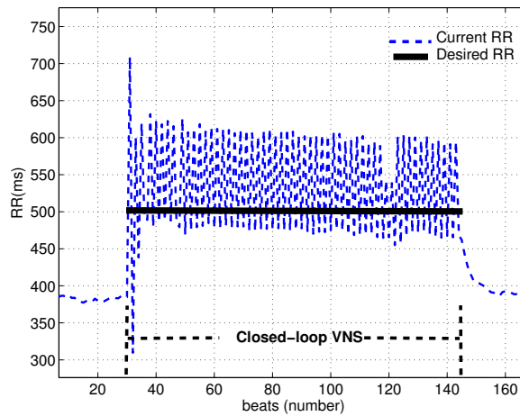
Fig. 3. RR interval when the minimal target RR = 500 ms with the stimulations parameters 3 mA and 2 pulses.
