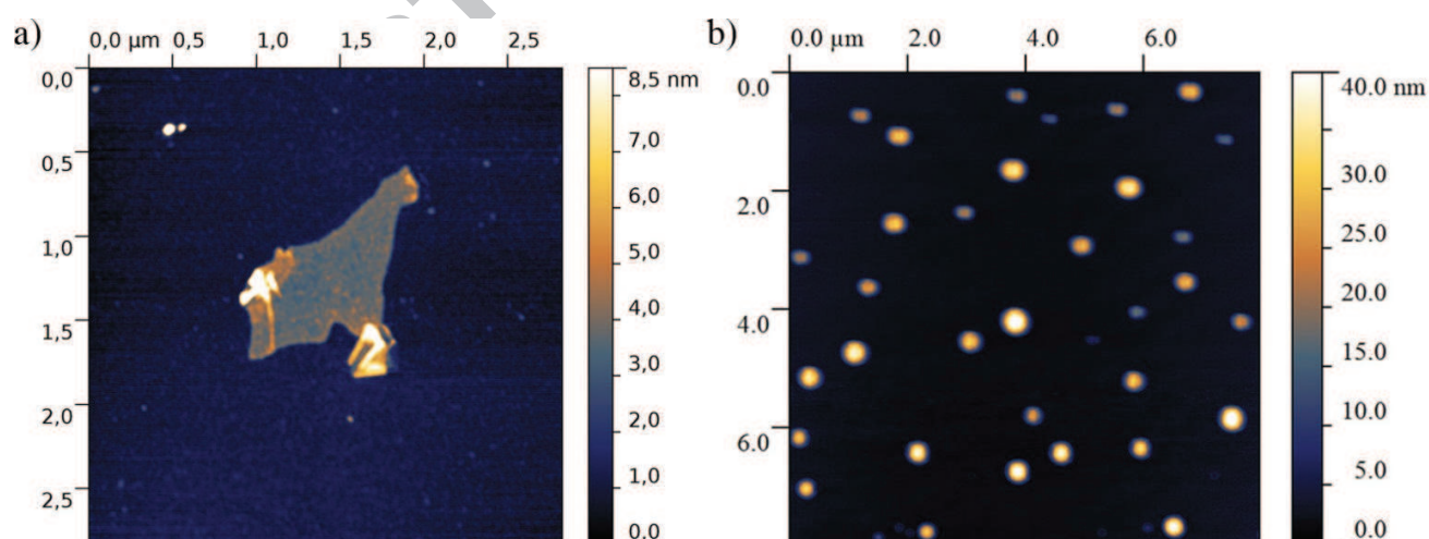
Figure 2. Typical AFM images of a representative a) graphene flak produce by electrochemical expansion of HOPG in DMF and b) carbon particles produce by electrochemical cathodic exfoliation of flexible graphite.
