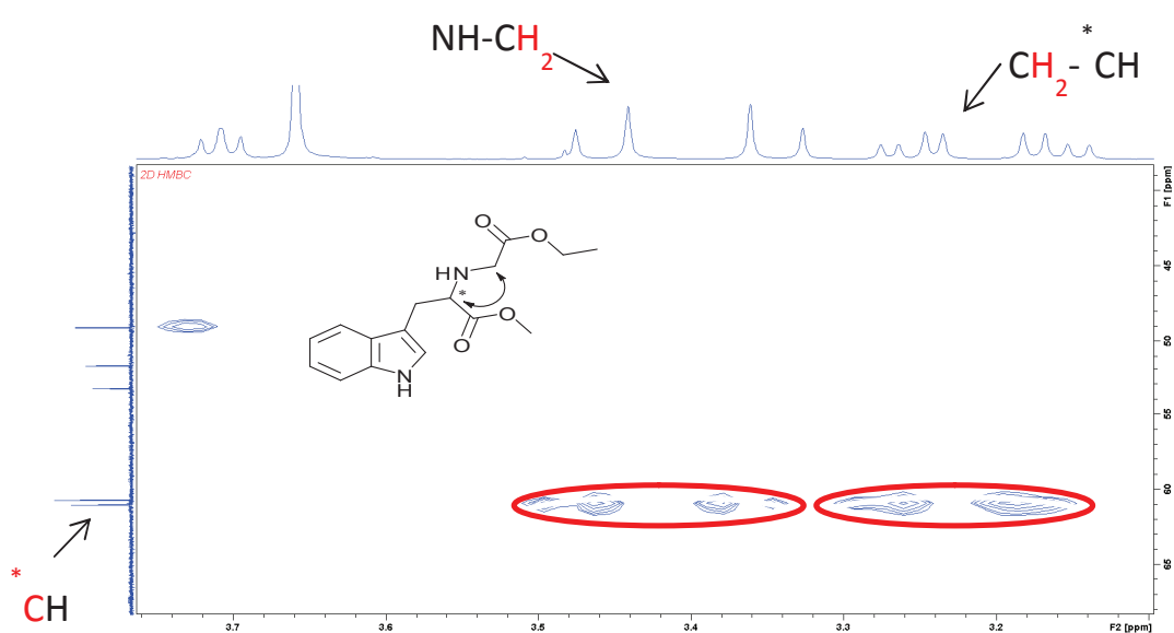
Fig. 2. ^1\text{H} - ^{13}\text{C} HMBC spectrum of ethyl diazoacetate insertion in N-H terminus bond of tryptophan.
