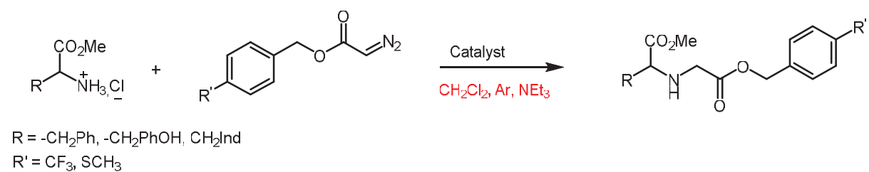
Scheme 2. Catalytic insertion of ethyl diazoacetate in N-H bond of amino esters.
