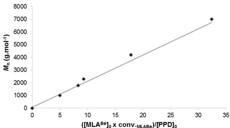
Figure 1. Variation of M_{n,NMR} (◆) and M_{n,theo} (solid line) values of PMLA Be , produced in the presence of Nd(OTf) 3 /PPD, as a function of ([MLA^{Be}]_0 \times \text{conv.MLABe}) / [PPD]_0 (Table 1, entries 4–8).
