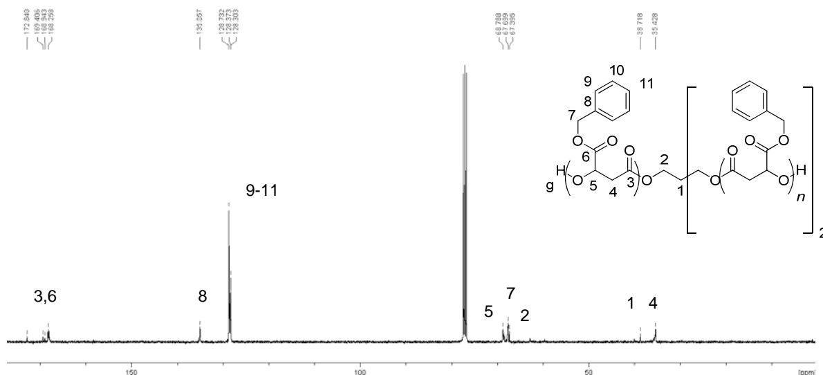
Figure 5. ^{13}\text{C}\{^1\text{H}\} NMR spectrum ( \text{CDCl}_3 , 125 MHz, 25 °C) of a \text{PMLA}^{\text{Be}} triol synthesized by ROP of \text{rac-MLA}^{\text{Be}} catalyzed by \text{Nd}(\text{OTf})_3 in presence of 5 equiv. of 2-hydroxymethyl-1,3-propanediol as initiator (Table 1, entry 10).
