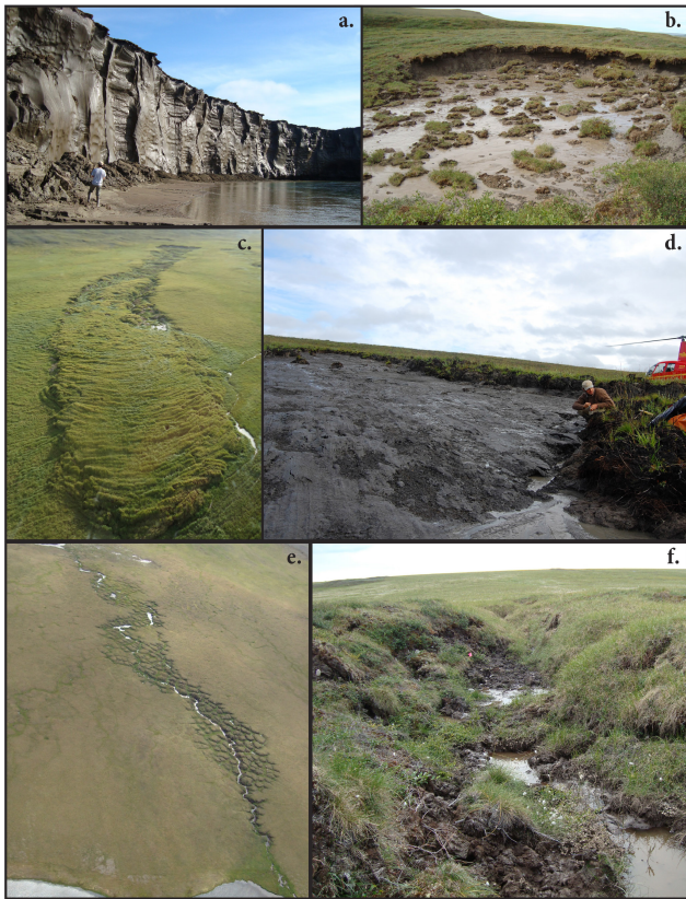
Figure 1. The three most common thermokarst morphologies in upland tundra: retrogressive thaw slumps (panels a , b ), active-layer detachment slides ( c , d ), and thermo-erosion gullies ( e , f ). Photo in panel ( c ) by A. W. Balsler.
