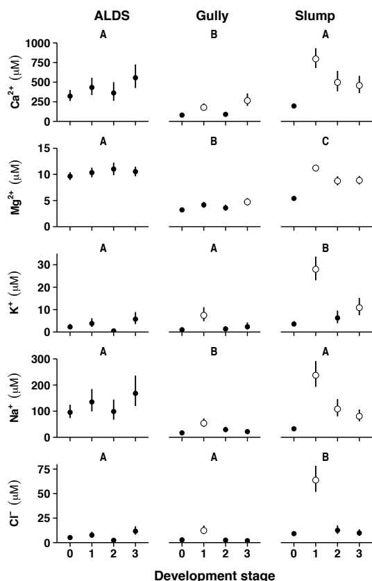
Figure 6. Major ion concentrations in outflow from 22 active-layer detachment slides, 19 thermo-erosion gullies, 42 thaw slumps, and 61 reference features. See Table 1 for complete definition of development stages: 0, reference; 1, most active; and 3, stabilized. Note log scales for \text{NO}_3^- and \text{NH}_4^+ . Symbology the same as Fig. 2.
