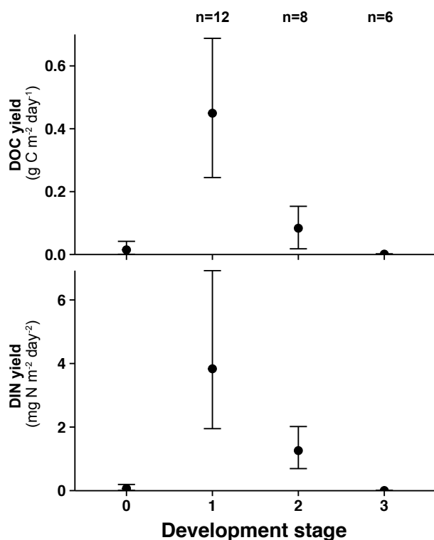
Figure 8. Geometric mean (SE) of dissolved organic carbon and dissolved inorganic nitrogen yield for thermokarst features in different development stages. Yield was calculated by difference in concentration above and below thermokarst feature multiplied by discharge and divided by feature area. Reference yields (stage 0) are maximum, minimum, and mean estimates from the literature for Arctic tundra (Giesler et al., 2014; McClelland et al., 2007; McClelland et al., 2014; Olefeldt et al., 2013; Peterson et al., 1993; Peterson et al., 1986; Townsend-Small et al., 2011). See Table 1 for complete definition of development stages: 0, reference; 1, most active; and 3, stabilized.
