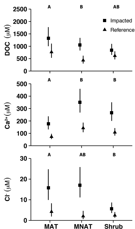
Figure 10. Mean ( \pm 95\% CI) of DOC for thermokarst outflow and reference water from sites occurring on moist acidic (MAT), nonacidic (MNAT), and shrub tundra. Different letters above panels represent significant differences between feature types. DOC, \text{Ca}^{2+} , and \text{Cl}^- were the only parameters for which vegetation was a significant predictor in the mixed-effects ANOVA when accounting for development stage, feature type, and landscape age.
