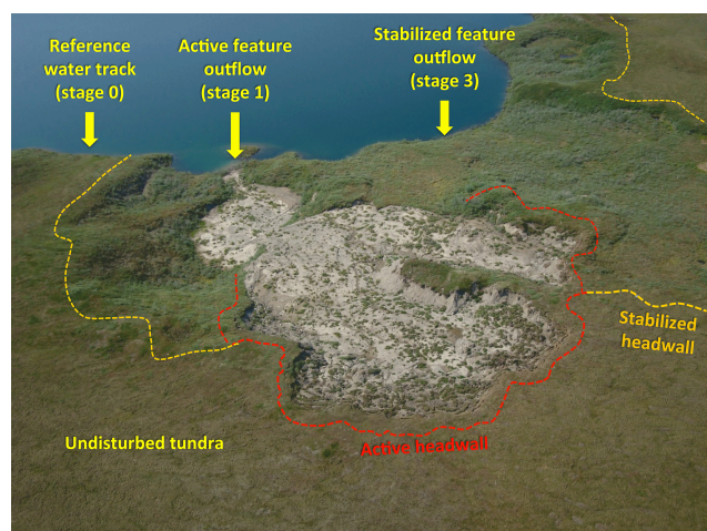
Figure 3. Aerial view of thaw slumps in various development stages. Samples were collected from feature outflows and adjacent water bodies such as unimpacted water tracks, streams, and lakes to assess the impact of thermokarst on water chemistry.
