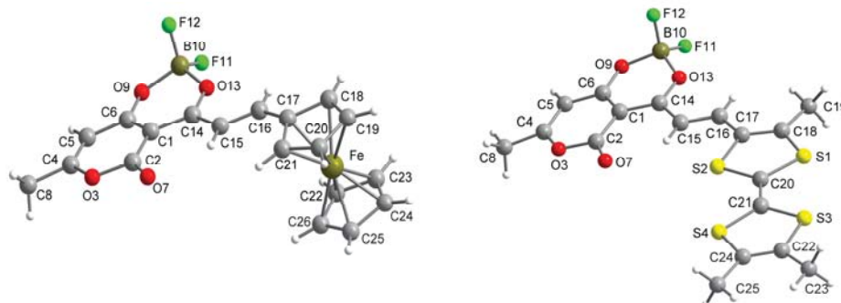
Fig. 1. Molecular structure of 5a (left), 5b (right)
