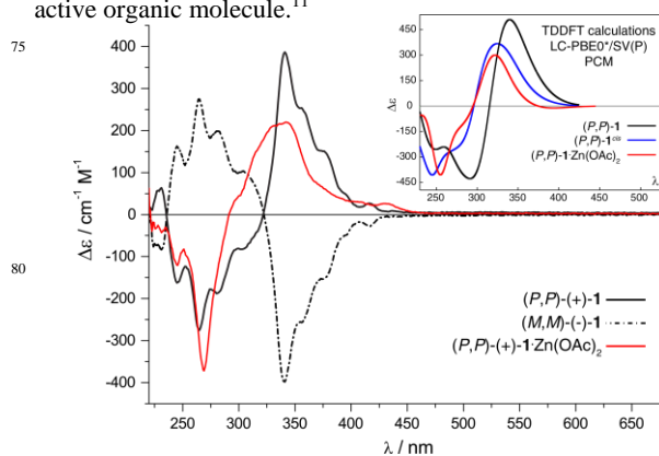
Figure 1. Experimental ECD spectra of enantiopure (M,M) - and (P,P) -1 and its Zn(II) complex (P,P) -1·Zn(OAc) 2 (CH 2 Cl 2 , 2 \times 10^{-5} \text{ M} ). Inset: Simulated spectra of (P,P) -1 ( trans and cis ) and (P,P) -1·Zn(OAc) 2 (see ESI).
