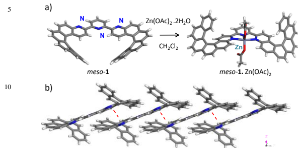
Scheme 2. a) Coordination of achiral ligand meso -1 to Zn 2+ , generating meso -1·Zn(OAc) 2 and their respective X-ray crystal structures. b) X-ray structure and supramolecular arrangement of (P,P) -1 along the x axis in the solid state.
