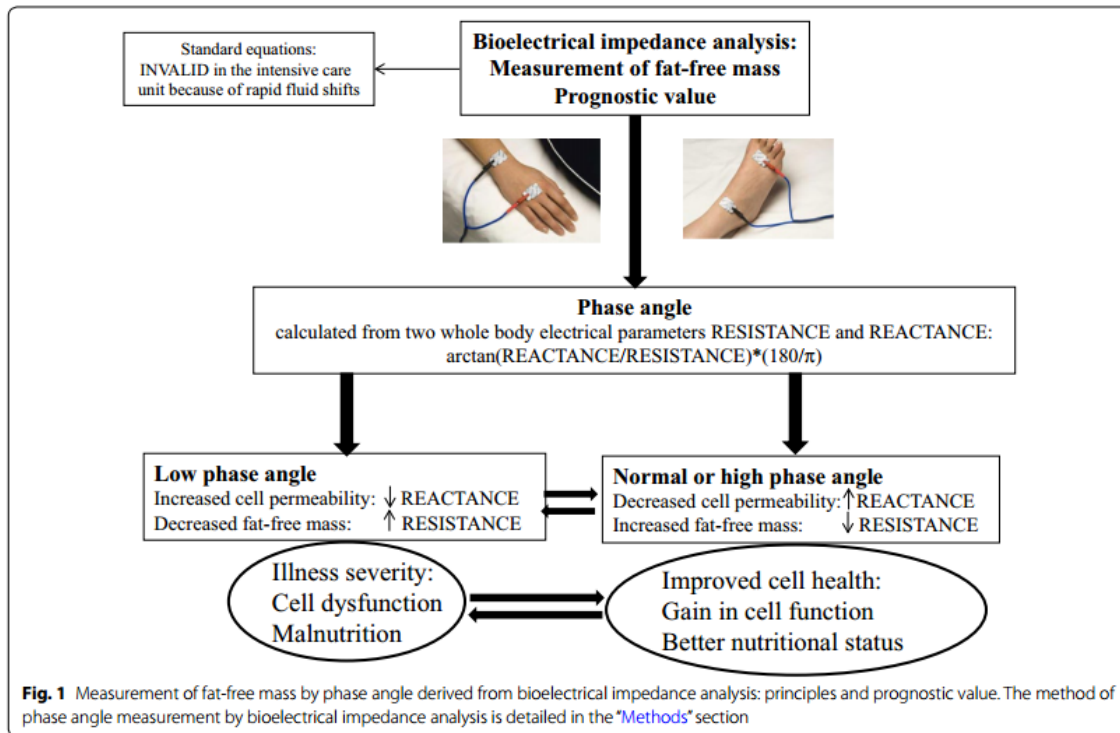
Figure 1 – Measurement of fat-free mass by phase angle derived from bioelectrical impedance analysis: principles and prognostic value. The method of phase angle measurement by bioelectrical impedance analysis is detailed in the dedicated paragraph of the ‘methods’ section.
