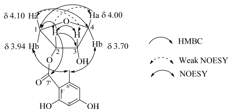
Fig. 4. Key HMBC and NOESY correlations of compound 5 .
