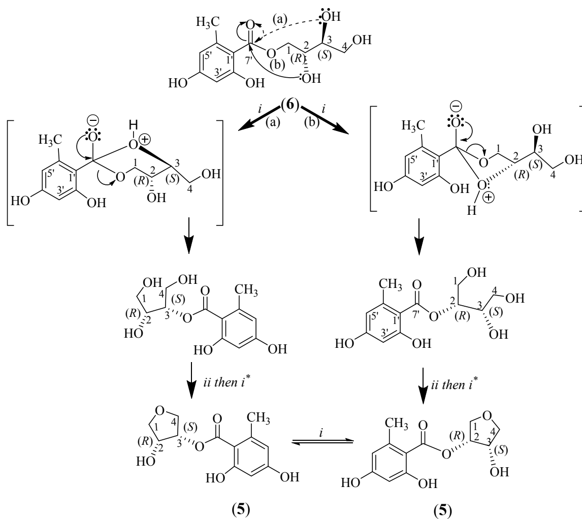
Scheme 1: The proposed biosynthetic pathway for the formation of compound 5 from D-montagnetol ( 6 ). [(i): transesterification; (ii): cyclodehydration].*or vice versa
