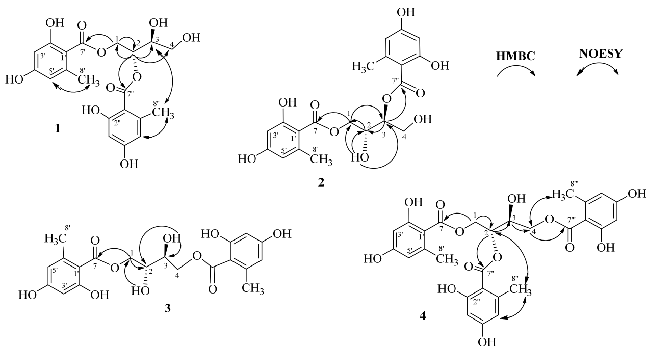
Fig. 2. Key HMBC and NOESY correlations of compounds 1–4
