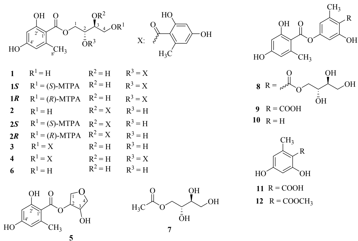
Fig. 1. Chemical structures of 1–12
