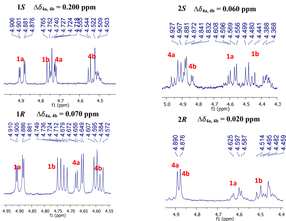
Fig. 3. Proton signal patterns of H 2 -4 of ( S )- and ( R )-MTPA esters of 1 ( 1S and 1R , respectively) (left) and 2 ( 2S and 2R , respectively) (right)
