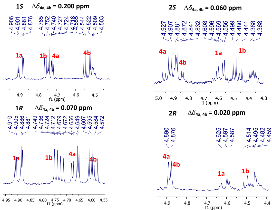
Fig. 3. Proton signal patterns of H 2 -4 of (S)- and (R)-MTPA esters ( 1S and 1R , respectively) (left) and ( 2S and 2R , respectively) (right)
