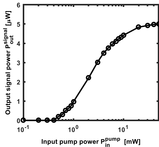
Fig. 16. Output signal power P_{out}^{signal} as a function of the input pump power P_{in}^{pump} with C_{Pr} = 10\,000 ppm and g_s = 4.3 \mu m.
