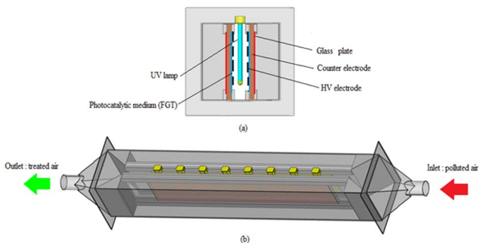
Figure 1. Schematic illustration of the used set-up: (a) sectional drawing and (b) planar reactor.
