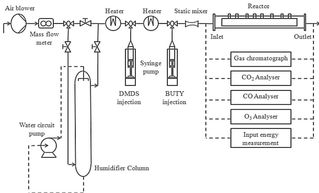
Figure 3. Experimental setup.
