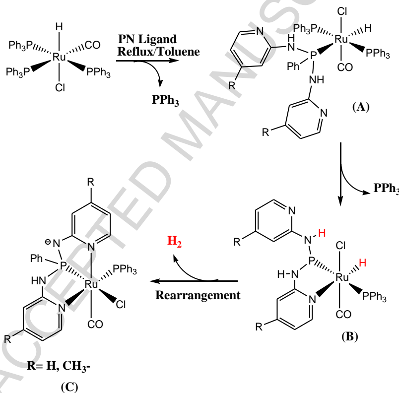
Scheme 2. Likely mechanism for the dehydrogenation of \text{Ru}(\text{Cl})(\text{CO})(\text{H})(\text{PPh}_3)_3 complex containing pincer-type ligands
