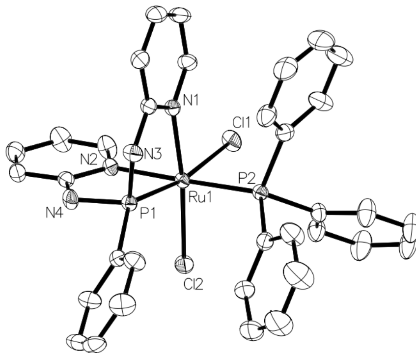
Figure 1 Crystal structure for complex 1
