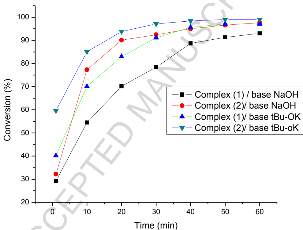
Figure 2. Catalytic activities of complexes \text{RuCl}_2\text{PPh}_3(\text{PPh}(\text{NHPy})_2) ( 1 ) and [\text{RuCl}_2\text{PPh}_3(\text{PPh}(\text{NHPyMe})_2)] ( 2 ) in the transfer hydrogenation of N-benzylideneaniline using different bases. Temperature 50 °C; substrate/catalyst ratio: 100/1.
