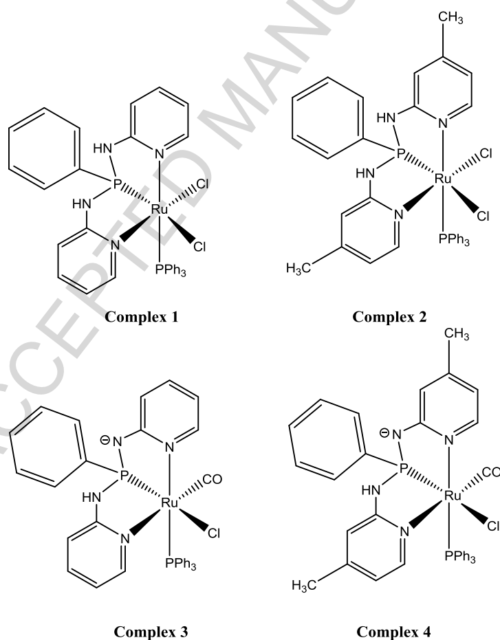
Scheme 1. Ruthenium complexes containing pincer-type phosphorus-nitrogen ligands(NPN) used as catalysts in the hydrogenation of N-benzylideneaniline.
