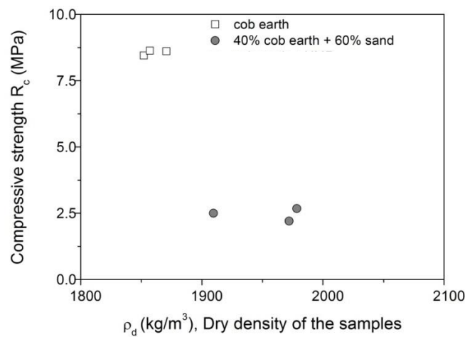
210 211 Fig. 5: Compressive strength as a function of dry density for cob earth with and without 212 additional sand.
