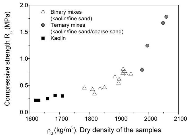
190 191 Fig. 4: Compressive strength as a function of dry density for kaolin, binary mix (fine 192 sand+kaolin) and ternary mix (coarse sand+fine sand+kaolin)
