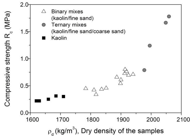
191 Fig. 4: Compressive strength as a function of dry density for kaolin, binary mix (fine 192 sand+kaolin) and ternary mix (coarse sand+fine sand+kaolin)
