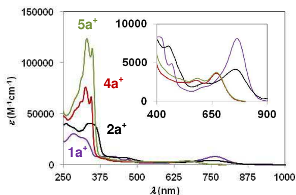
Figure 3. UV-Vis absorption spectra for 1a [ \text{PF}_6 ], 2a [ \text{PF}_6 ], 4a [ \text{PF}_6 ] and 5a [ \text{PF}_6 ] in \text{CH}_2\text{Cl}_2 at 25\text{ }^\circ\text{C} .
