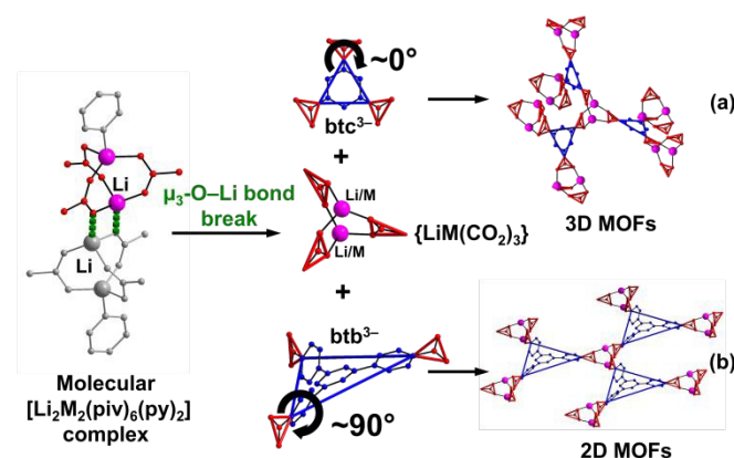
Scheme 2. General representation of {LiM} building block formation and construction of coordination polymers with different dimensionality depending on the position of carboxylic group in plane of the ligand (a) forming a 3D framework or out of the plane (b) forming hcb layered structure.
