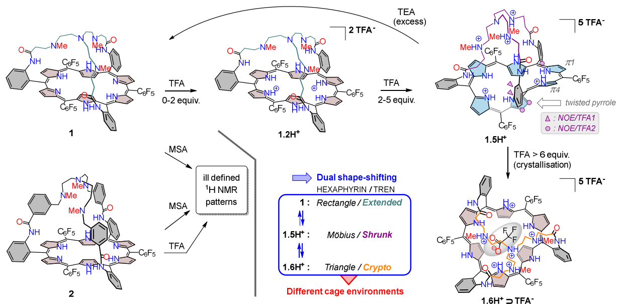
Scheme 1. Protonation study of tren-capped hexaphyrins 1 and 2 with TFA and MSA, and induced conformational changes (NMR study at low temperature in \text{CD}_2\text{Cl}_2 or \text{CDCl}_3 ).
