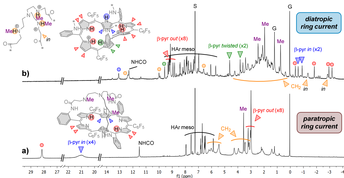
Figure 2. 1 H NMR spectra of 1 (a) and 1.5H + (b, scale * 2) ( \text{CDCl}_3 , 500 MHz, 233 K). S = solvent, G = grease.
