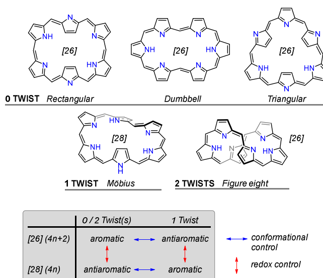
Figure 1. Main conformations of regular hexaphyrins (independently of their [26/28] oxidation state) and interplay between conformation, oxidation state and (anti)aromaticity.
