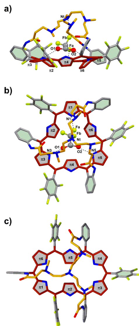
Figure 3. Crystallographic structure of compounds 1.6H + TFA - ; (a) side and (b) top views, and 1 (c), top view. 5 H atoms, solvents of crystallization, and exo -TFA molecules removed for clarity. Hexaphyrin highlighted in dark brown and tren cap in orange, endo -TFA depicted in ball-and-stick. Dashed lines indicate H bonds.
