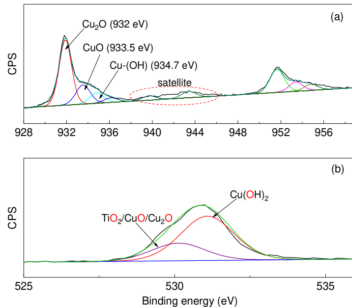
Figure 8. XPS deconvolution of (a) \text{Cu}2p and (b) \text{O}1s at the topmost layers of \text{Cu}_x\text{O}/\text{TiO}_2 -PES surface: species in direct contact with the pollutants and the bacteria.
