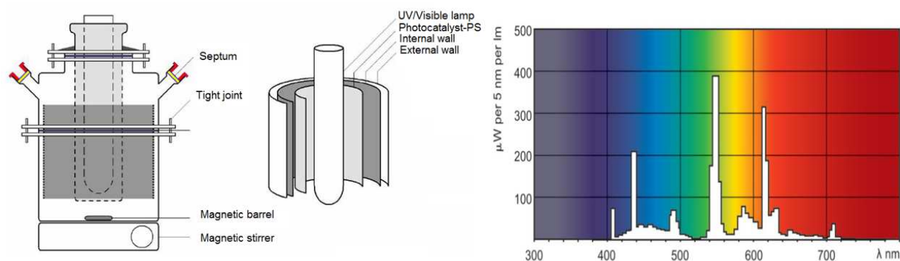
Figure 1. Schematic of the batch photo-reactor with the central co-axial Sylvania CF-L 24W/840 light source (400-720 nm).
