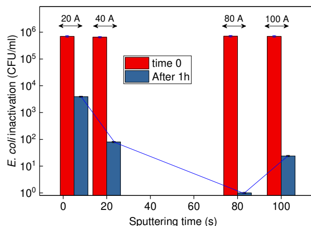
Figure 6. E. coli inactivation on Cu x O/TiO 2 -PES under low intensity indoor light.
