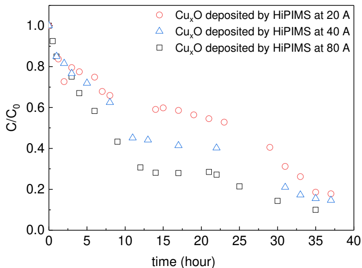
Figure 2. Removal of chloroform with catalyst \text{Cu}_x\text{O}/\text{TiO}_2\text{-PES} at different HiPIMS sputtering currents deposited for 100 s.
