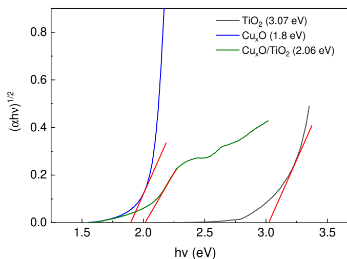
Figure 7. Tauc's plot for band-gaps estimation of: (1) \text{TiO}_2 , (2) \text{Cu}_x\text{O} and (3) \text{Cu}_x\text{O}/\text{TiO}_2 deposited by HiPIMS on polyester.
