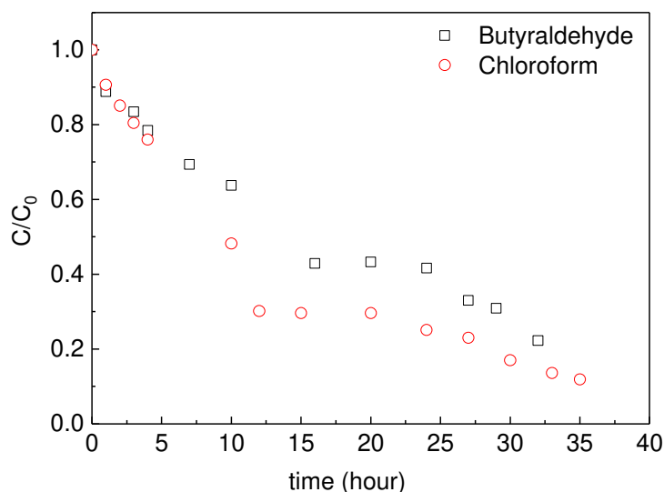
Figure 4. Indoor/outdoor pollutants removal on \text{Cu}_x\text{O}/\text{TiO}_2 -PES HiPIMS-sputtered 80 A for 20s under a visible lamp irradiation.
