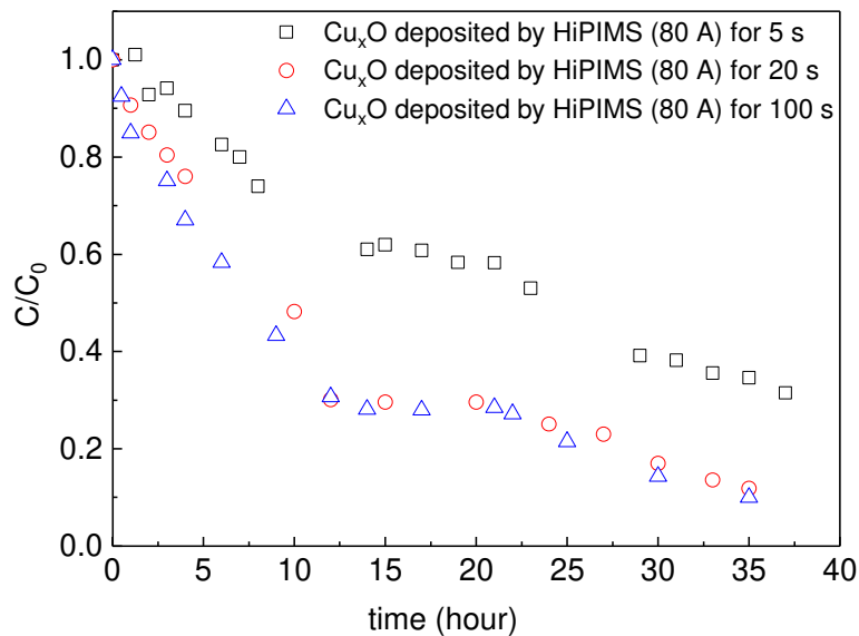
Figure 3. Removal of chloroform on HiPIMS-sputtered \text{Cu}_x\text{O}/\text{TiO}_2\text{-PES} (at 80 A) deposited at different times.
