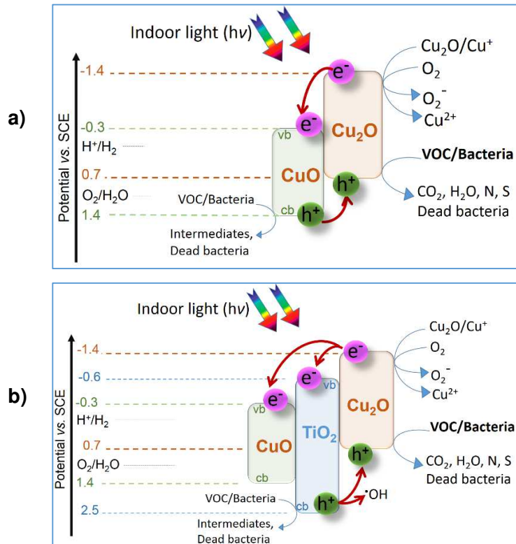
Figure 9. Proposed mechanisms of action of the prepared photocatalyst: (a) if we consider just \text{Cu}_x\text{O} interface, (b) if we consider a photocatalytic intervention of the \text{TiO}_2 under layer.
