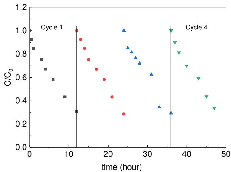
Figure 5. Degradation profile of chloroform with photocatalysis on a \text{Cu}_x\text{O}/\text{TiO}_2\text{-PES} sample under visible light. Further experimental conditions: I=30\text{W}/\text{m}^2 , Chloroform concentration = 6\text{ g}/\text{m}^3 .
