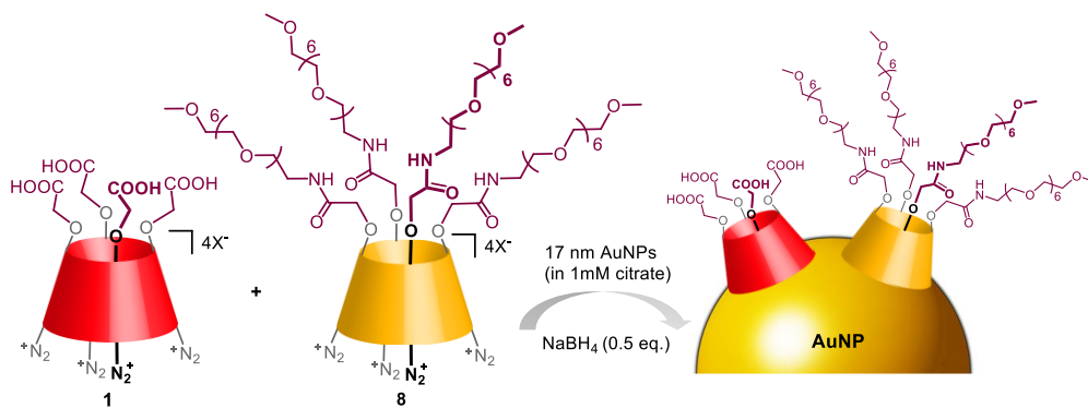
Figure 10. Schematic representation of the grafting of calix[4]arenes 1 and 8 on citrate-protected AuNPs in aqueous solutions.
