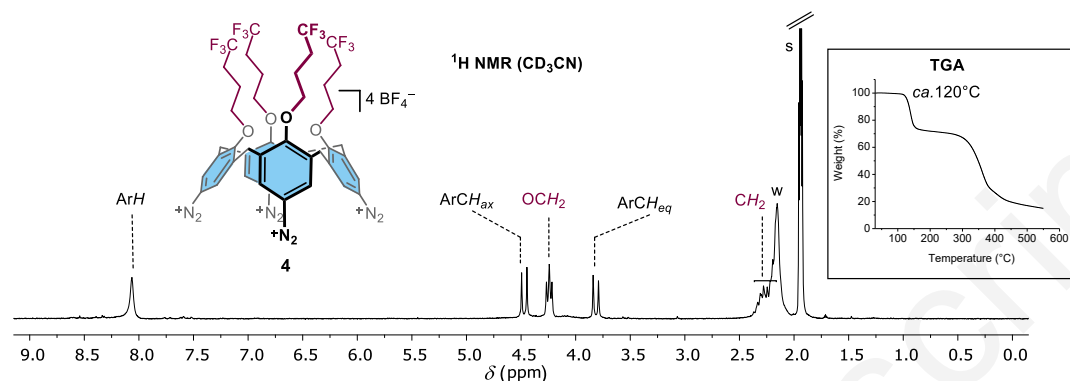
Figure 5: 1 H NMR (CD 3 CN, 300 MHz) spectrum of C 4v symmetrical calix[4]arene tetradiazonium 4 . Inset: thermogravimetric analysis of 4 . 58
