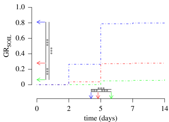
Figure 2. Germination rate of the progeny ( GR_{SOIL} ) in soil at different time points (days) according to geographical origin. The dot-dashed lines indicate the dynamic of the germination for the three geographical areas: Asia (green, GR = 0.07 ), Europe (red, GR = 0.28 ), Middle East (blue, GR = 0.81 ). The vertical arrows indicate the mean germination time, and the horizontal arrows indicate the portion of germination for each geographical area. The asterisks indicate significant differences between the three regions ( *p < 0.05 ; **p < 0.01 ; ***p < 0.001 ). (Online version in colour.)
